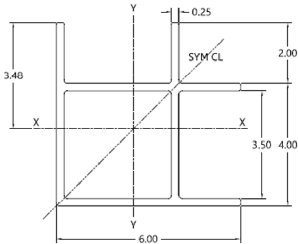
SQUARE CORNER POST AREA = 5.77 IN 2 WEIGHT = 6.93 LBS/FT MOMENT OF INERTIA = 20.16 IN 4 SECTION MODULUS = 5.79 IN 3
