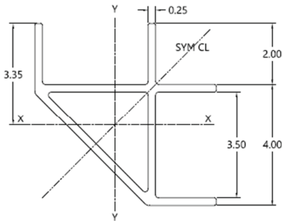
CORNER POST AREA = 5.11 IN 2 WEIGHT = 6.32 LBS/FT MOMENT OF INERTIA = 8.58 IN 4 SECTION MODULUS = 2.56 IN 3
