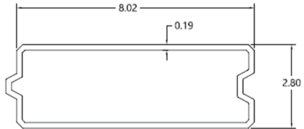
BUILDABLE BOX PANEL AREA = 4.63 IN 2 WEIGHT = 4.84 LBS/FT MOMENT OF INERTIA = 5.50 IN 4 SECTION MODULUS = 3.93 IN 3
