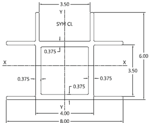
MIDDLE T-POST AREA = 8.44 IN 2 WEIGHT = 10.14 LBS/FT MOMENT OF INERTIA = 27.29 IN 4 SECTION MODULUS = 7.49 IN 3
